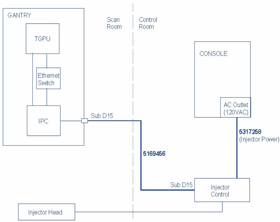
Figure 3-1 Interconnect Diagram
